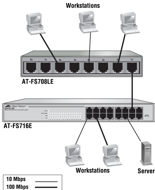
Figure 4 Cascade Topology
