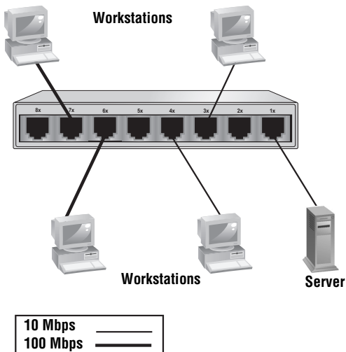
Figure 3 Standalone Topology
